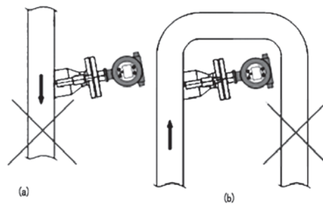
Schematic diagram of unreasonable installation of vertical pipelines
