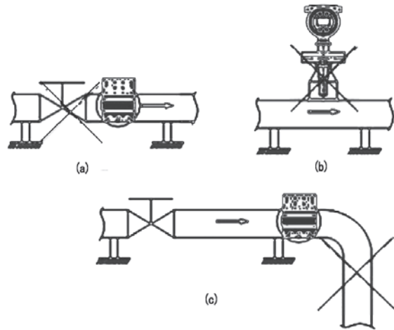
Schematic diagram of unreasonable installation of horizontal pipeline
