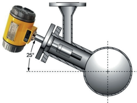
Instrument installation for open tanks (long pole)
